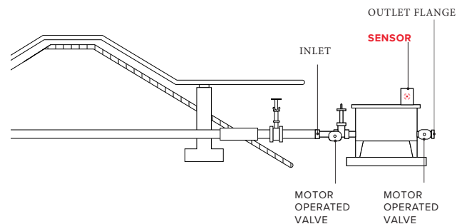
Dike Outfalls
